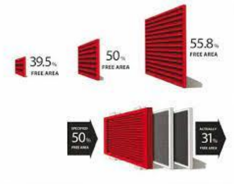
Figure 2: Free Area of Louvers of Construction Specialties
